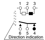
2-coil latching
