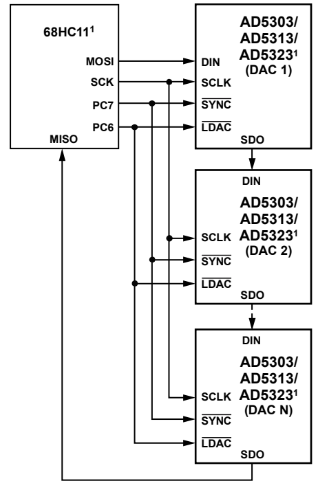
Figure 46. Daisy-Chain Mode
