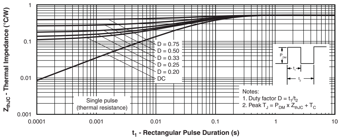
Fig. 3 - Maximum Thermal Impedance Z_{thJC} Characteristics
