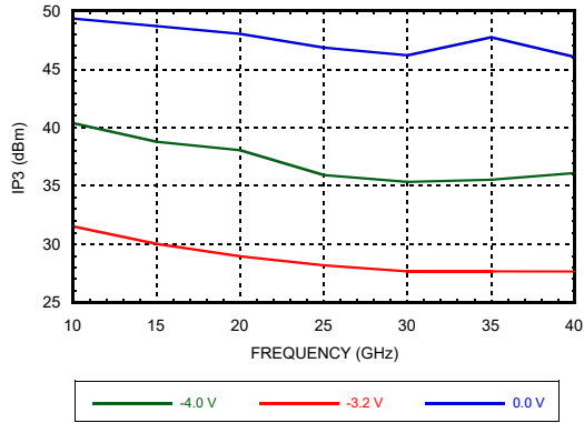
Input IP3 vs. Frequency Vctrl1 = Vctrl2
