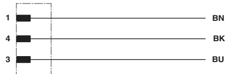
Contact assignment of the M5 connector
