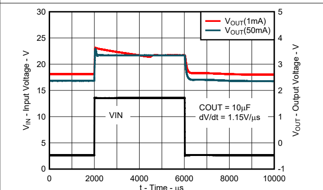
Figure 8-10. TPS71533-Q1 Dropout Exit Transient Response for New Chip
