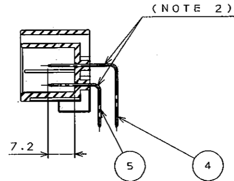
SECT. B-B
