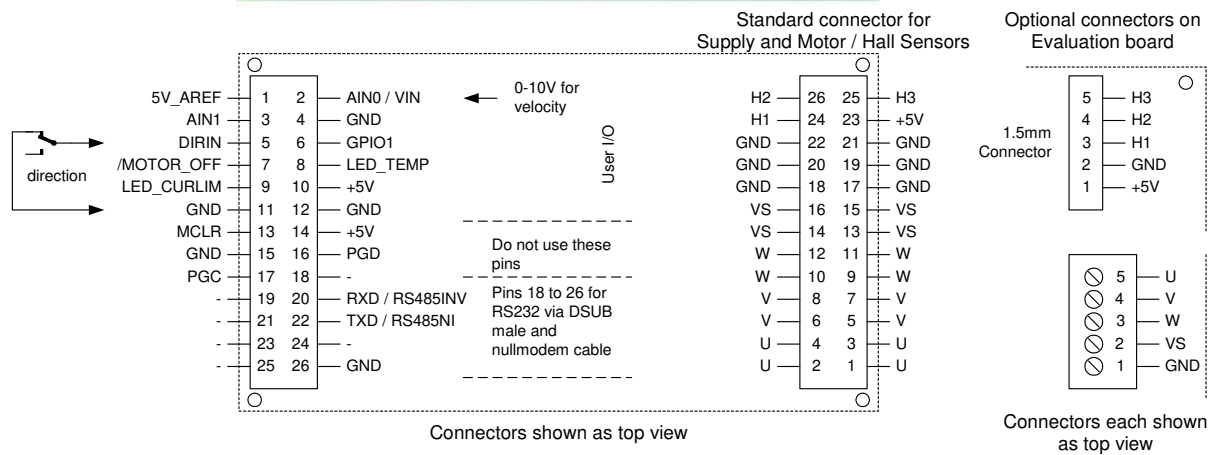
Figure 3.1: Pinning
