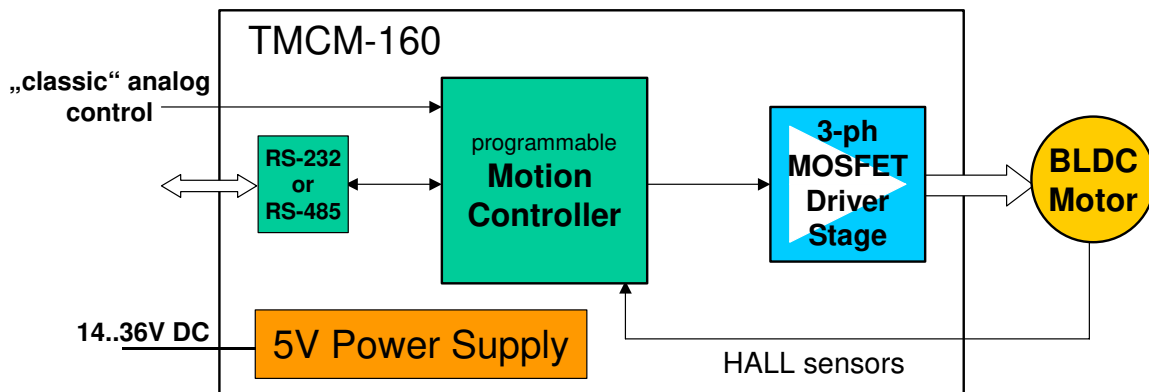
Figure 3.3: Application Environment
