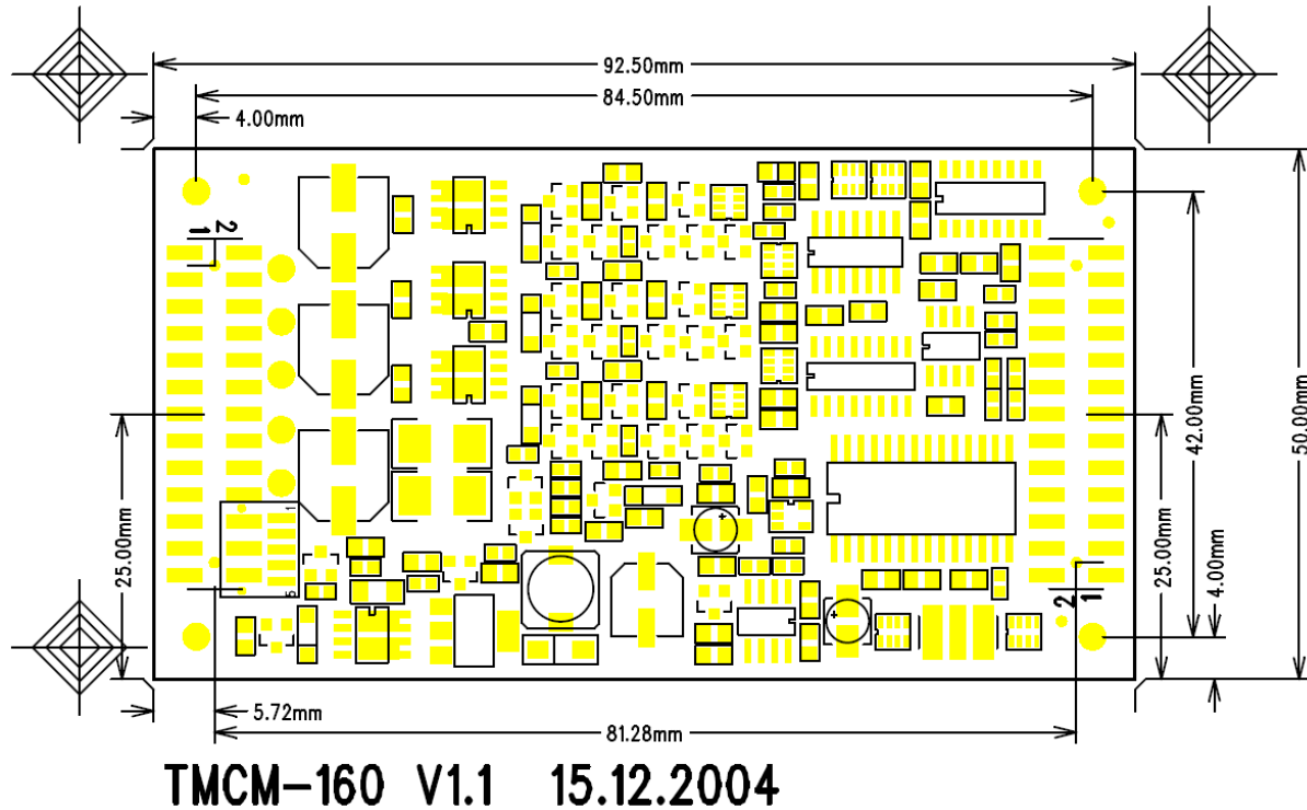
Figure 3.2: Dimensions
