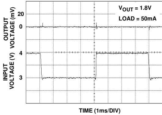
FIGURE 3. LINE REGULATION RESPONSE ( V_{OUT1} )
