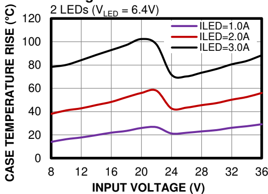
Case Temperature Rise vs. Input Voltage
