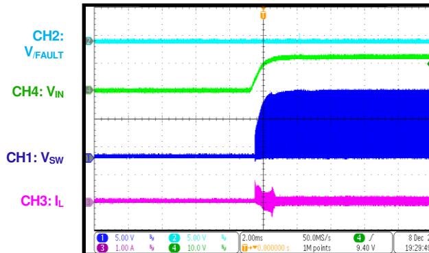
LED Open Input Start-Up
