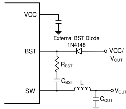
Figure 6: Optional External BST Diode to Enhance Efficiency
