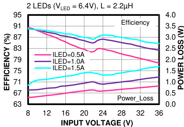
Efficiency vs. Input Voltage vs. Power Loss
