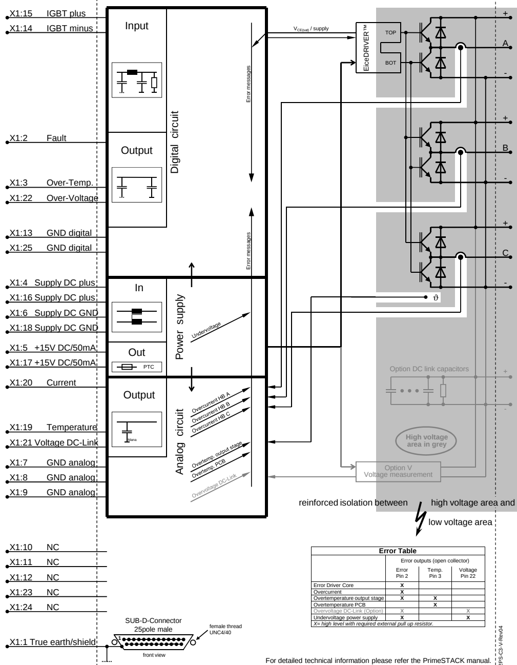
Circuit diagram
