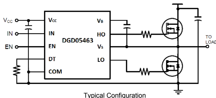
W-DFN3030-10
