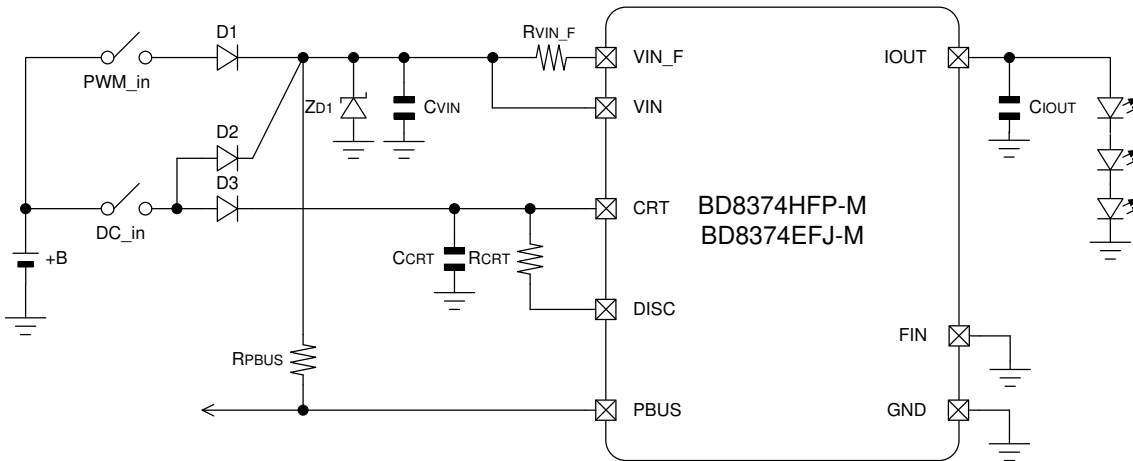
Figure 27. Recommended Application Circuit
