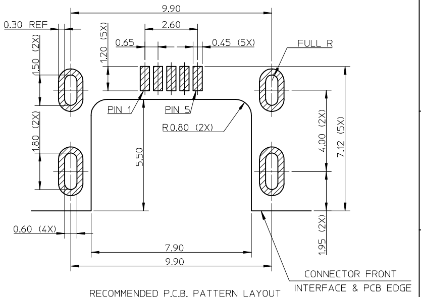
RECOMMENDED P.C.B. PATTERN LAYOUT GENERAL TOLERANCE: ±0.05
