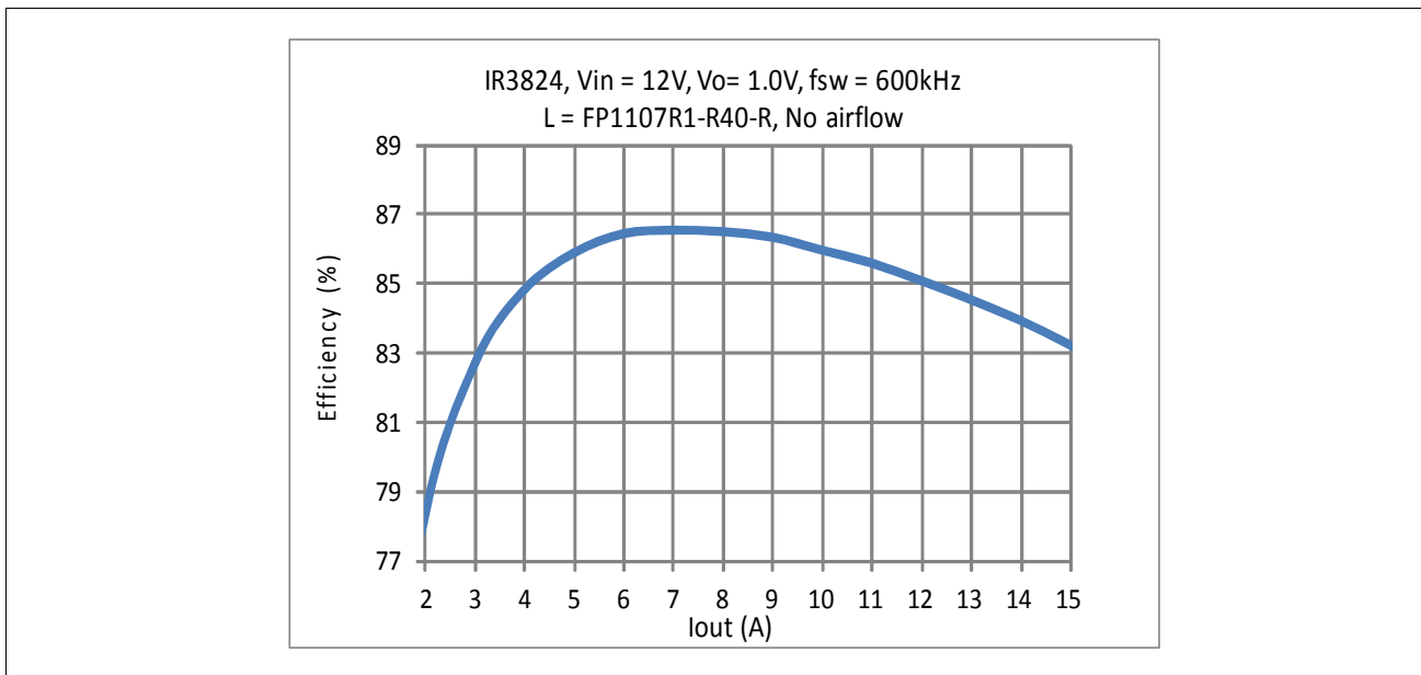
Figure 2-2 IR3824 Efficiency
