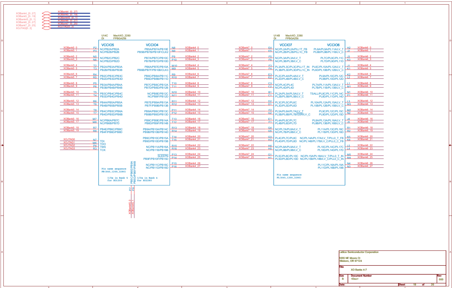
Figure 22. MachXO Banks 4 to 7
