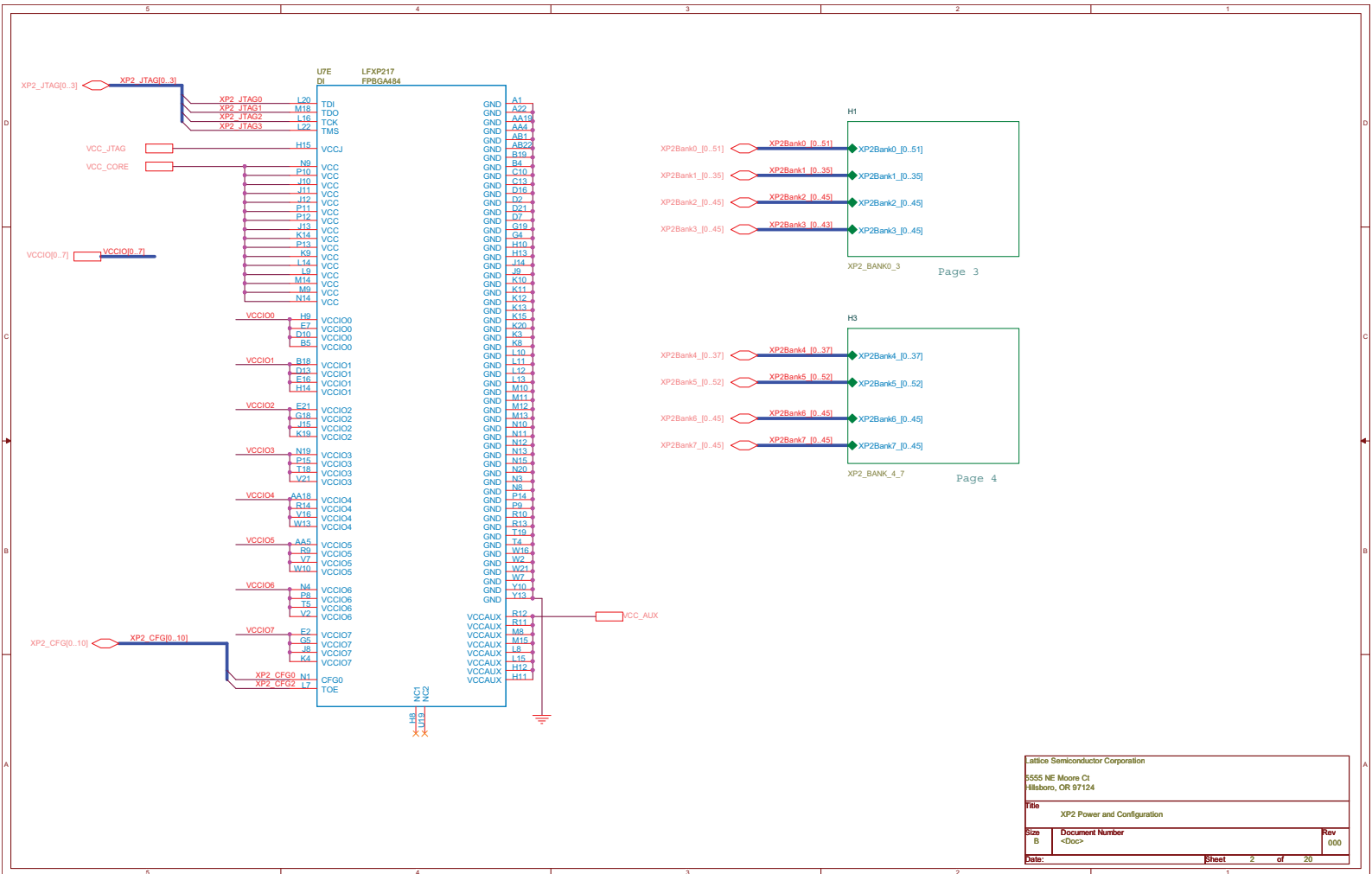
Figure 5. LatticeXP2 Power and Configuration
