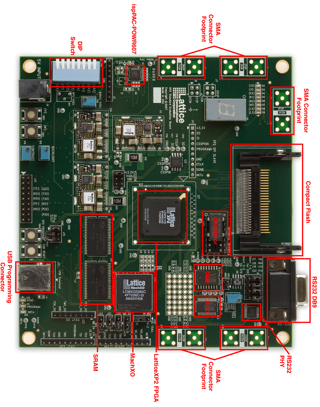
Figure 1. LatticeXP2 Standard Evaluation Board
