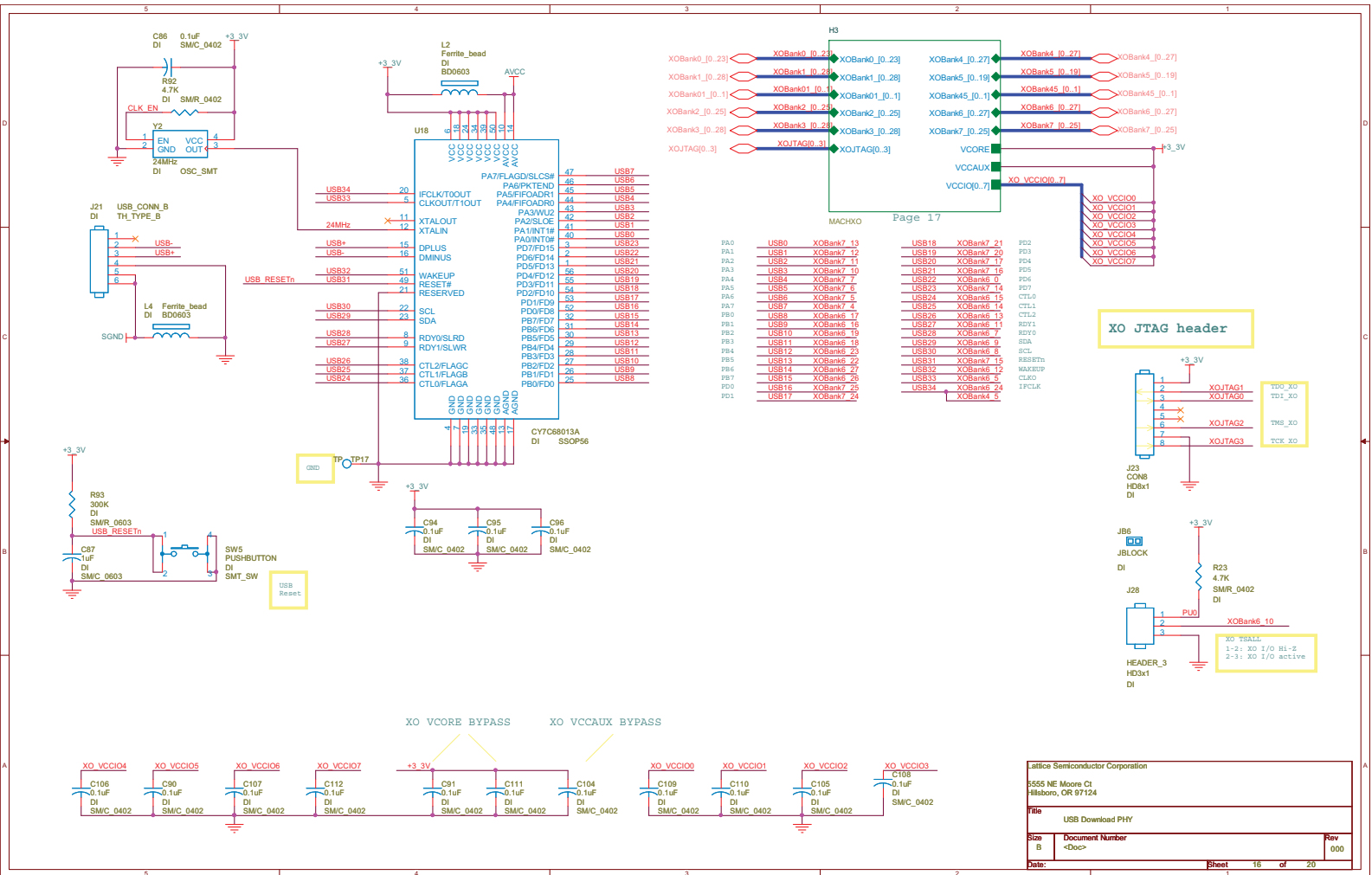
Figure 19. USB Download PHY
