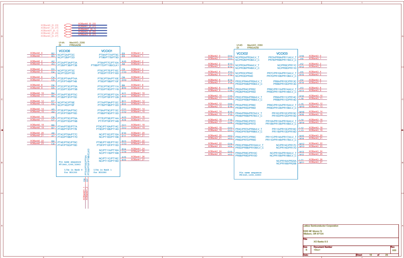
Figure 21. MachXO Banks 0 to 3
