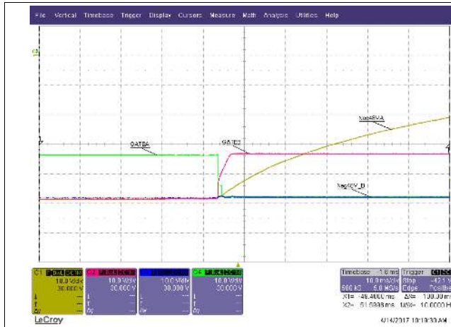
V_{IN,A} = 54.5\text{ V} ; V_{IN,B} = 54\text{ V} , I_{load} = 5\text{ A} , scope GND=RTN
