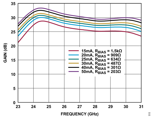
Figure 11. Gain vs. Frequency for Various I_{DQ} and R_{BIAS} Values, V_{DD} = 2 V
