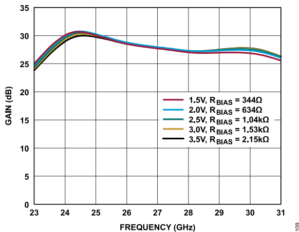
Figure 9. Gain vs. Frequency for Various Supply Voltages and R_{BIAS} Values, I_{DQ} = 25 mA
