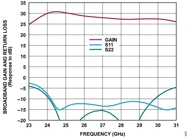
Figure 7. Broadband Gain and Return Loss vs. Frequency, V_{DD} = 2 V , I_{DQ} = 25 mA
