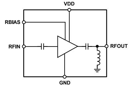
Figure 63. Simplified Schematic
