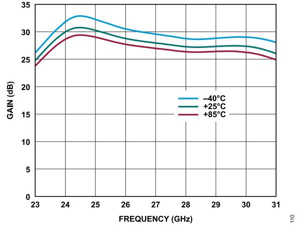
Figure 10. Gain vs. Frequency for Various Temperatures, V_{DD} = 2 V , I_{DQ} = 25 mA , R_{BIAS} = 634 \Omega
