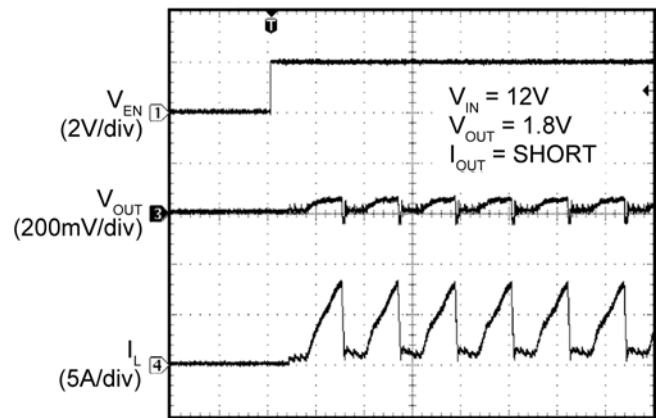
Time (100µs/div)
