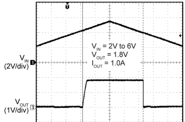
Time (20ms/div)
