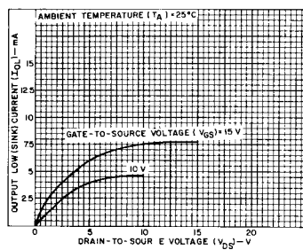
Fig. 9 - Minimum n-channel output low (sink) current characteristics.
