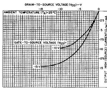
Fig. 10 - Typical p-channel output high (source) current characteristics.
