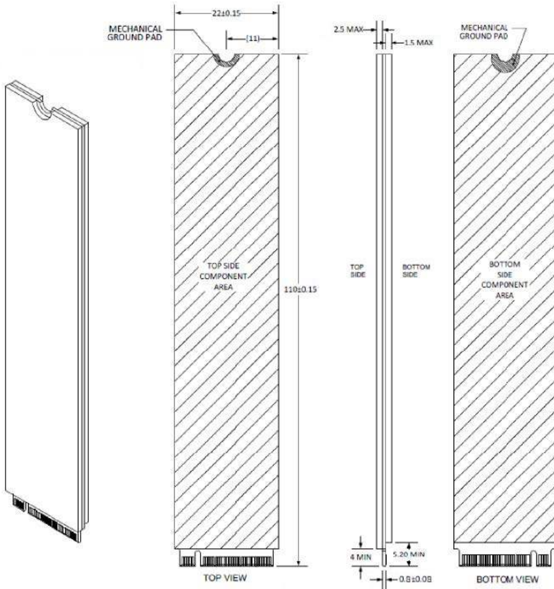
Figure 4: Nominal Dimensions
