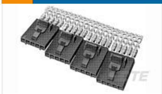
TE Part # 103961-9 2X10 MTE RCPT SR LATCH .100CL
