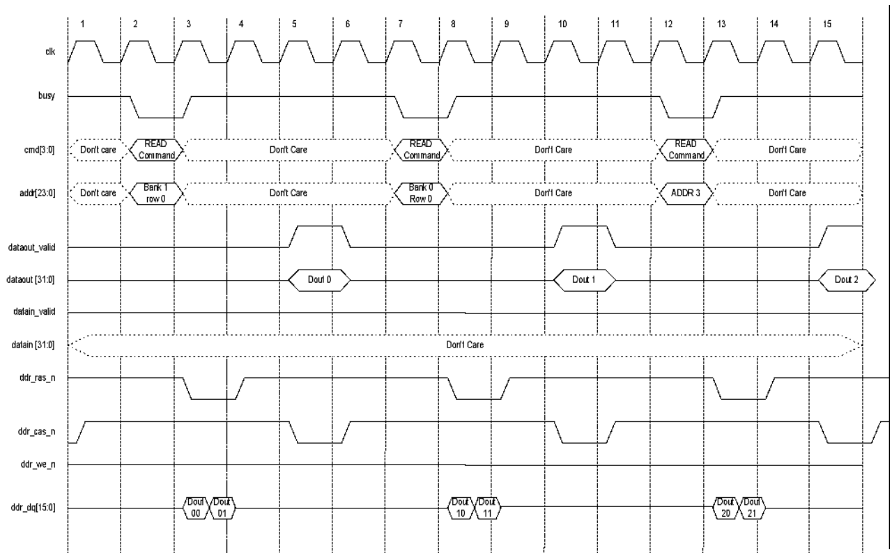
Figure 8. Read Followed by Read (Different Bank Row Open BL = 2)
