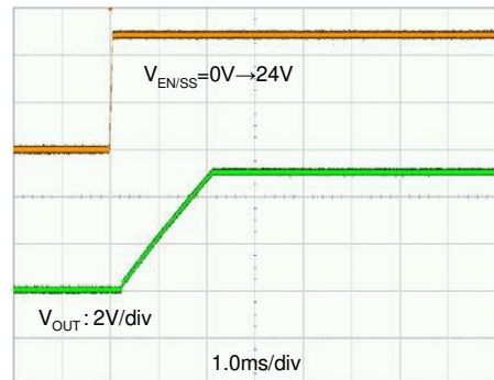
MYRGC075060W31RA V_{IN}=24V , V_{EN/SS}=0V \rightarrow 24V ( t_r=50\mu s ), V_{OUT}=5.0V , I_{OUT}=300mA C_{IN1}=4.7\mu F , C_{IN2}=0.1\mu F , C_L=22\mu F
