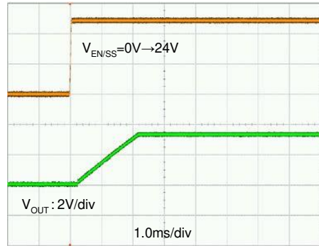
MYRGC075060W31RA V_{IN}=24V , V_{EN/SS}=0V \rightarrow 24V ( t_r=50\mu s ), V_{OUT}=3.3V , I_{OUT}=300mA C_{IN1}=4.7\mu F , C_{IN2}=0.1\mu F , C_L=22\mu F
