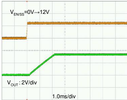
MYRGC075060W31RA V_{IN}=12V , V_{EN/SS}=0V \rightarrow 12V ( t_r=50\mu s ), V_{OUT}=3.3V , I_{OUT}=300mA C_{IN1}=4.7\mu F , C_{IN2}=0.1\mu F , C_L=22\mu F
