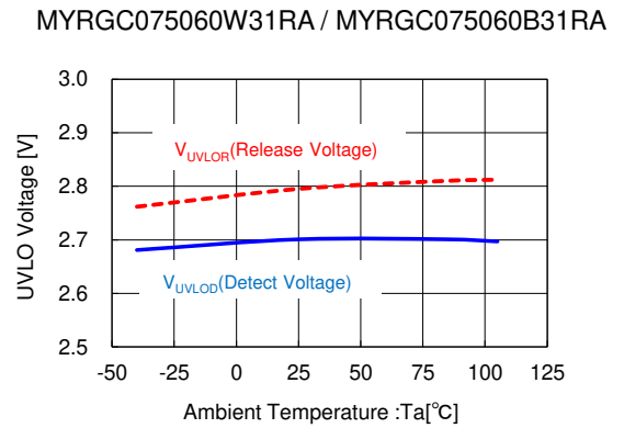
(5) UVLO Voltage vs. Ambient Temperature
