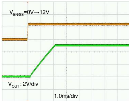
MYRGC075060W31RA V_{IN}=12V , V_{EN/SS}=0V \rightarrow 12V ( t_r=50\mu s ), V_{OUT}=5.0V , I_{OUT}=300mA C_{IN1}=4.7\mu F , C_{IN2}=0.1\mu F , C_L=22\mu F
