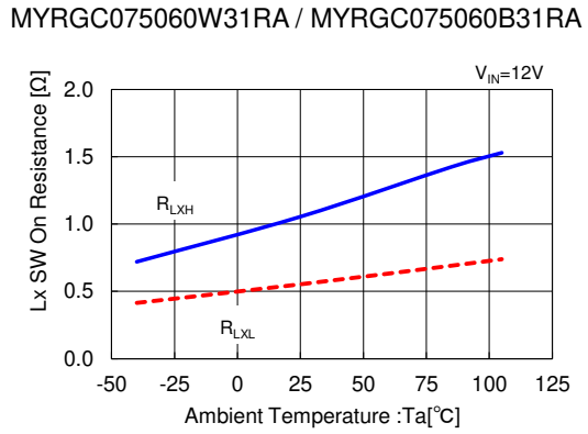
(7) Lx SW On Resistance vs. Ambient Temperature
