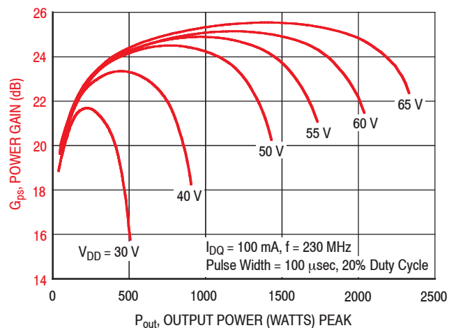
Figure 21. Power Gain versus Output Power and Drain-Source Voltage
