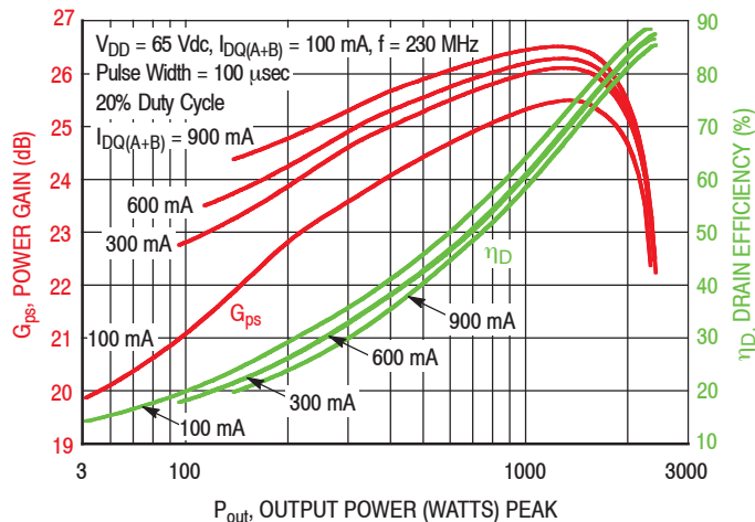
Figure 19. Power Gain and Drain Efficiency versus Output Power and Quiescent Current
