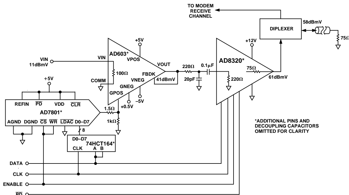
Figure 47. Enhanced Dynamic Range Circuit
