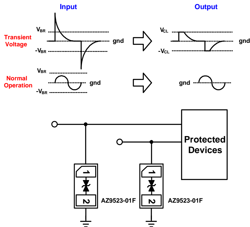
Fig. 1 ESD protection scheme by using AZ9523-01F.
