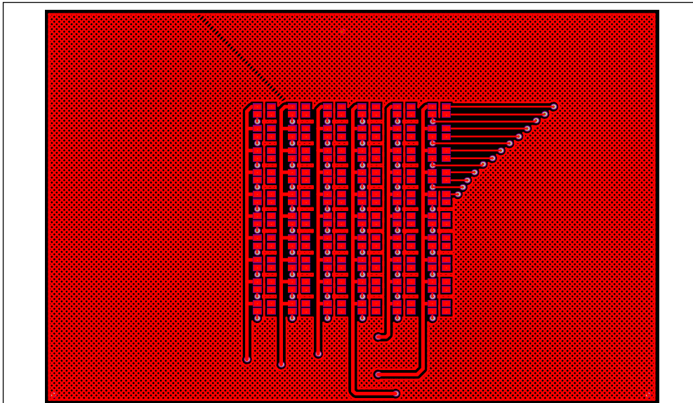
Figure 10: LED Board PCB Layout - Top Layer
