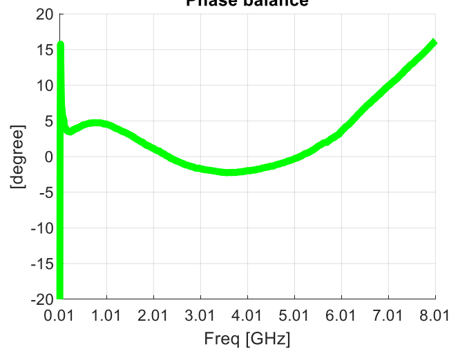
Phase balance
