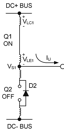
Figure 26: V_S positive
