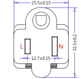
ME-307 (NEMA 5-15R) (Dimensions of Connector Face)
