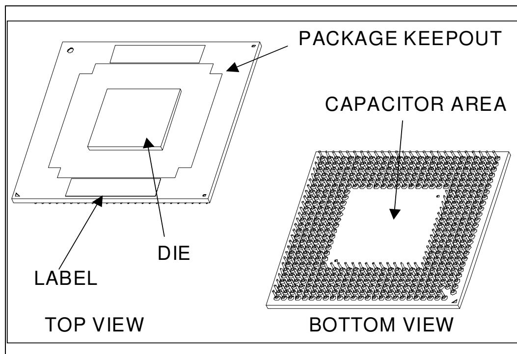
Figure 4-1. Micro-FCPGA Package Top and Bottom Isometric Views
