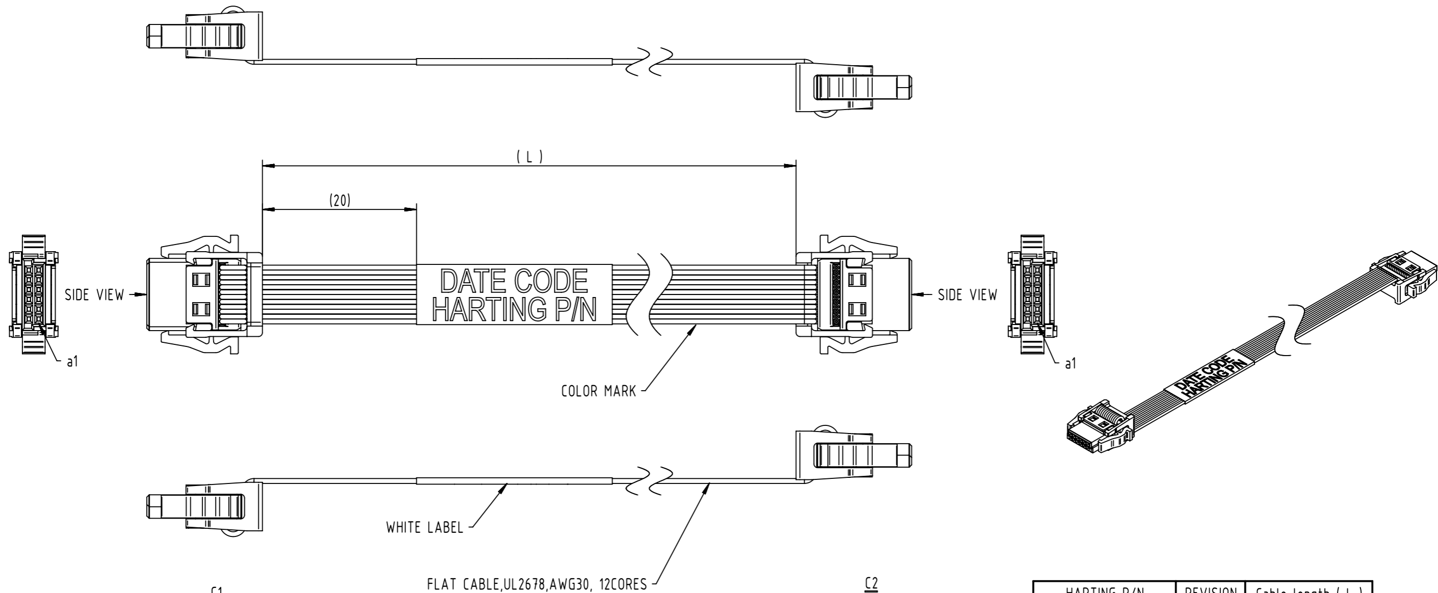
C1 HAR-FLEX 12 POLES FEMALE CONNECTOR WITH STRAIN RELIEF
