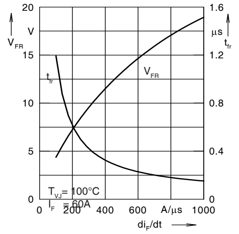
Fig. 23 Peak forward voltage V_{FR} and t_{rr} versus di_F/dt
