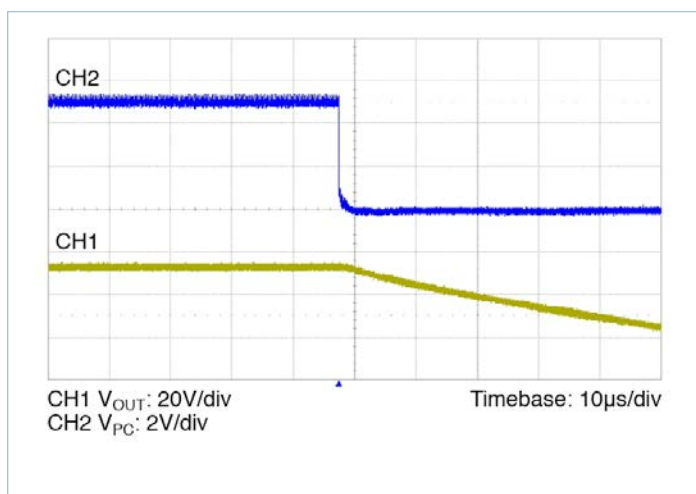
Figure 17 — PC disable waveform, 270V V_{IN} , 100 \mu F C_{OUT} full load
