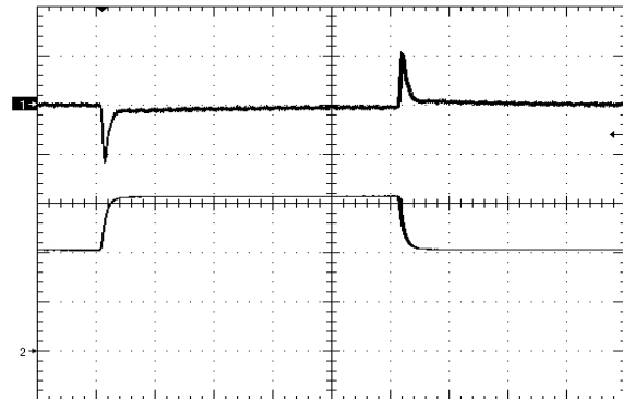
Figure 10. Load Transient Response (100mV/div), di/dt=0.1A/uS, 50% - 75% - 50% of full load, time scale: 200uS/div
