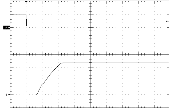
Figure 8. Startup Waveform via Enable Pin, time scale 10mS/div. Vin=Vin_nom, full res. load + 4700uF, negative enbl, Ch1=5V/div, Ch2=5V/div
