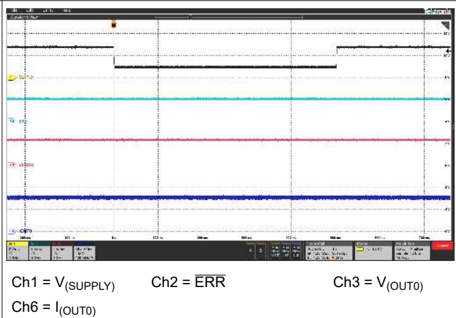
Figure 7-14. Transient Undervoltage
