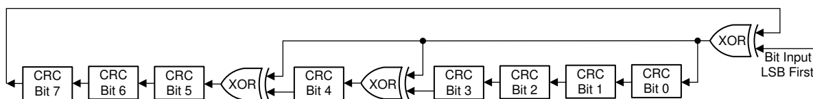
Figure 8-7. CRC Algorithm Diagram
