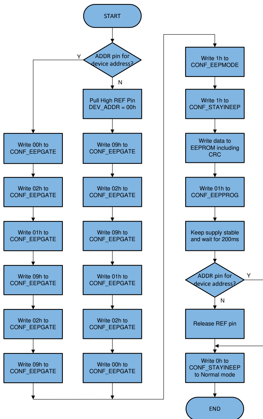
Figure 8-18. Programming Sequence
