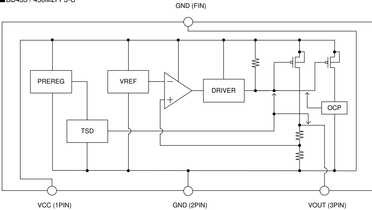
Figure 4. Block Diagrams
