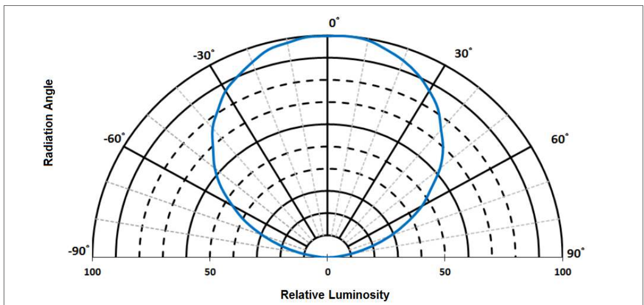
Figure 8: Typical Polar Radiation Pattern at 125mA, T_{sp}=25^{\circ}\text{C}
