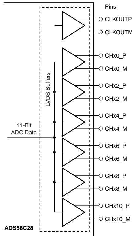
Figure 64. DDR LVDS Interface
