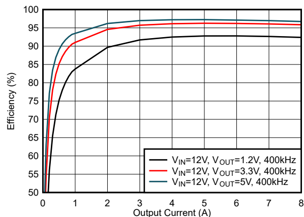
Efficiency, FCCM Mode
