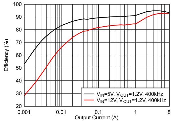
Figure 6-11. Efficiency, Mode = DCM, f_{SW} = 400\text{ kHz}
