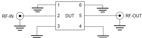
Fig 1. Block diagram of Test Circuit used for characterization, Test board TB-QAT-9C+ Conditions: Attenuation, VSWR: Pin=0 dBm
