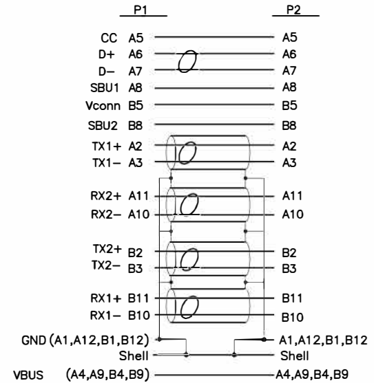
Pin Assignment
