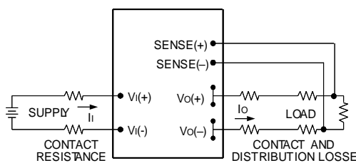
Figure 11. Circuit Configuration for remote sense .
