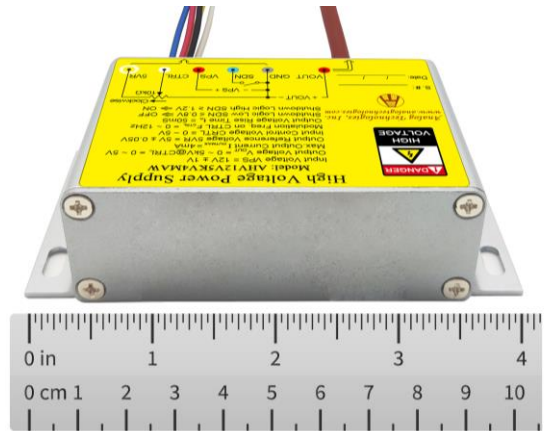
Figure 1.3. Side View
