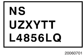
Top View NS - Std NS Logo U - Wafer Fab Code Z - Assembly Plant Code XY - 2 Digit Date Code TT - Die Run Traceability L4856LQ - LM4856LQ
