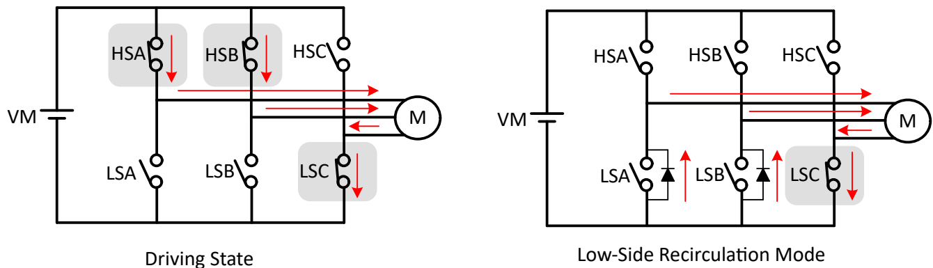
Figure 7-45. Low-Side Recirculation
