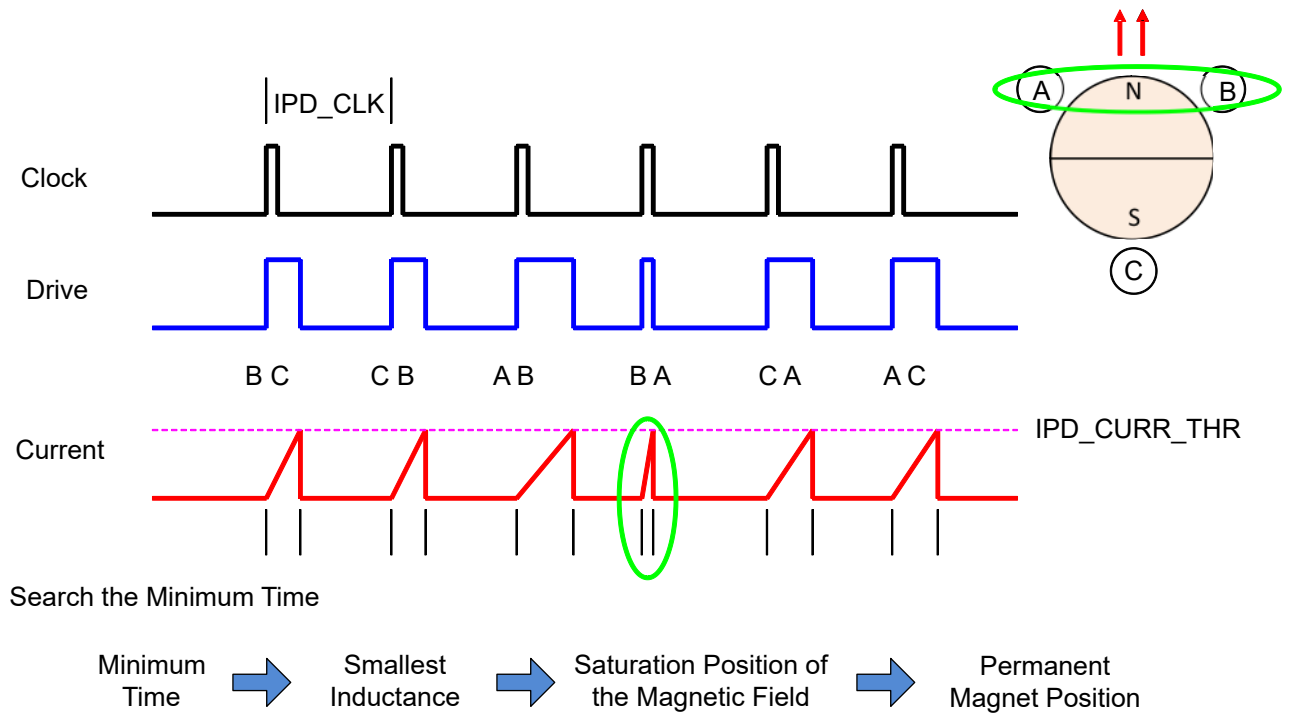
Figure 7-26. IPD Function
