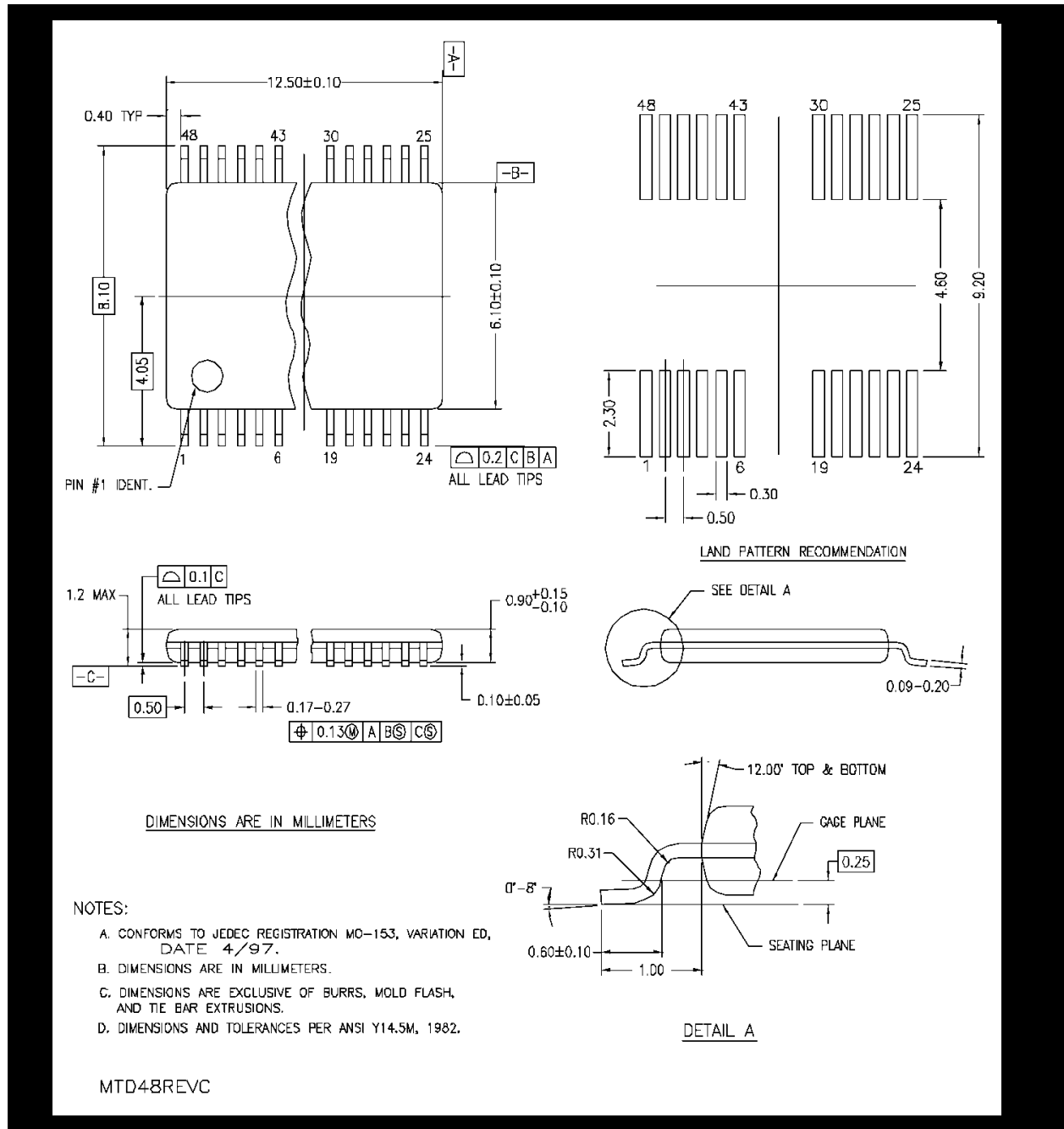
Figure 6. 48-Lead Thin Shrink Small Outline Package (TSSOP), JEDEC MO-153, 6.1mm Wide Package Number MTD48
