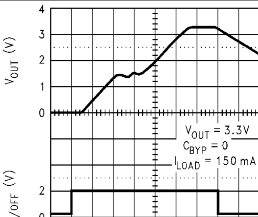
Figure 35. Turn-On Time
