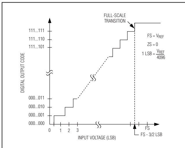
Figure 4a. MAX1377/MAX1379 Unipolar Transfer Function ( \bar{U}/B = Low )
